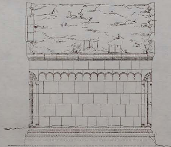
GOSHAVANK THE LUSAVORICH CHURCH FACADES
