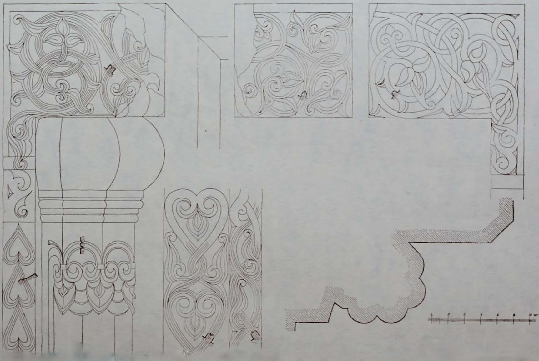
GOSHAVANK THE LUSAVORICH CHURCH DETAILS OF THE PORTAL
