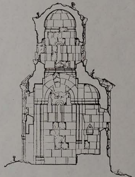
GOSHAVANK SAINT GEORGE CHURCH SECTIONS
