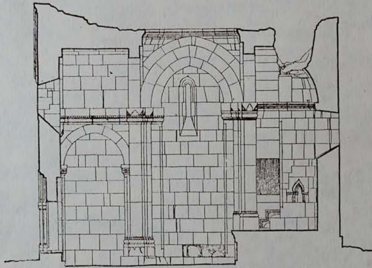
SAINT GREGORY TEMPLE LONGITUDINAL SECTIONS
