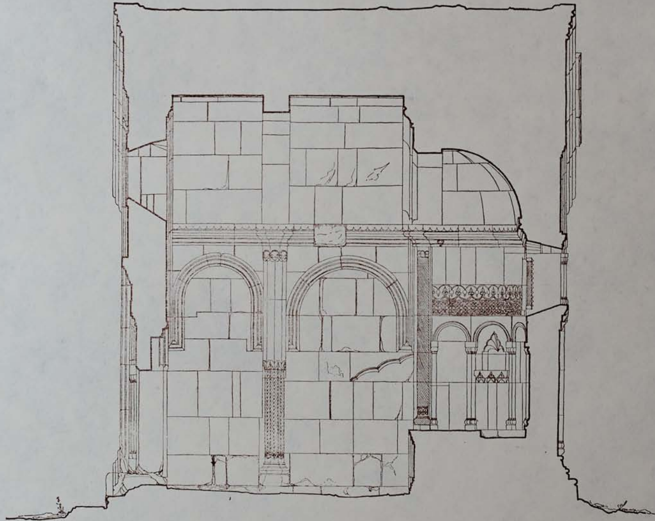
GOSHAVANK THE LUSAVORICH CHURCH LONGITUDINAL SECTION
