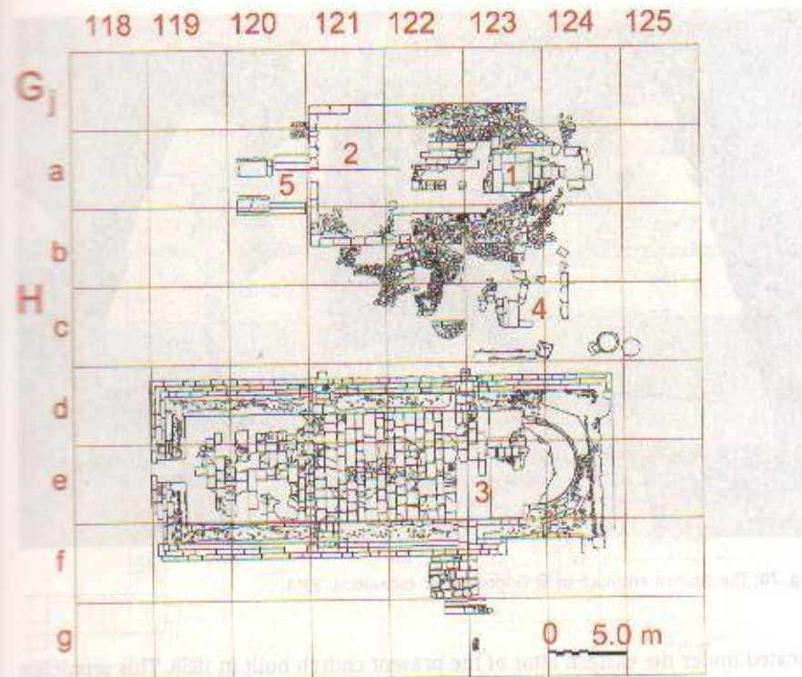
Fig. 19: Plans of Early Christian structures: 1) Sepulchre, 2) Small church, 3) Large church, 4) Monument, 5) Graveyard, 2014.
