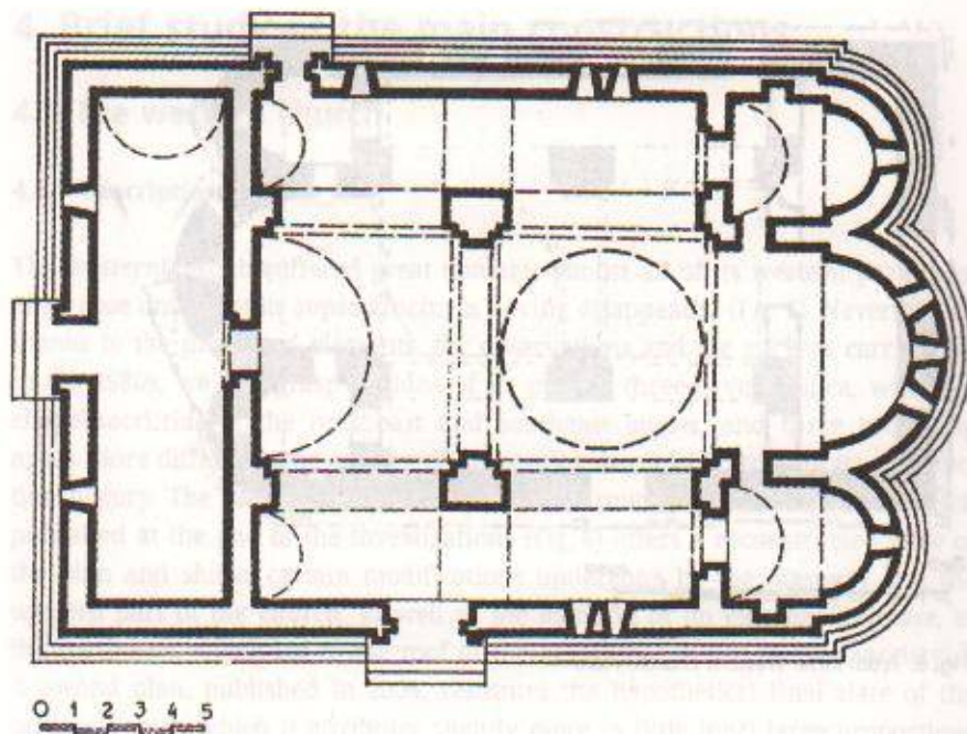
Fig. 7: Yeddi Kilsa. Western church. Plan.
